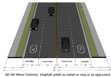
60'-66' Minor Collector (Asphalt width as noted on map or as approved)
