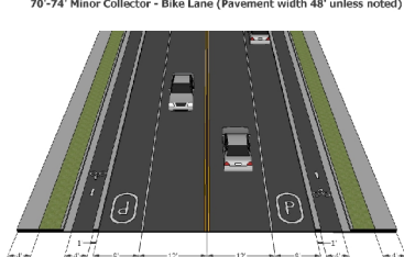
70' Minor Collector - Cycle Track (1700 W)
