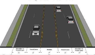
80' Major Arterial
