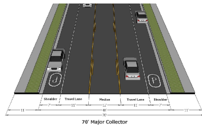
70' Major Collector
