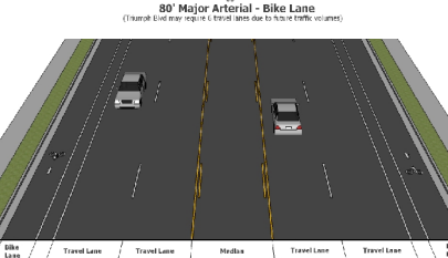
102' Major Arterial - Buffered Bike Lane
