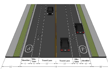
66' Minor Collector - Bike Lane
