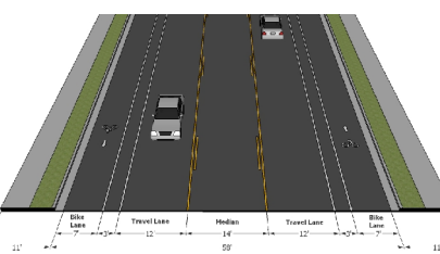
80' Major Collector - Buffered Bike Lane
