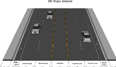
80' Major Arterial - Bike Lane (Through bike lanes only. Arterial bike lanes due to 15-ft or more clearance)
